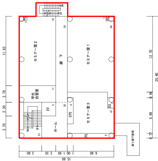
3階平面図 S = 1/300 (324㎡)
